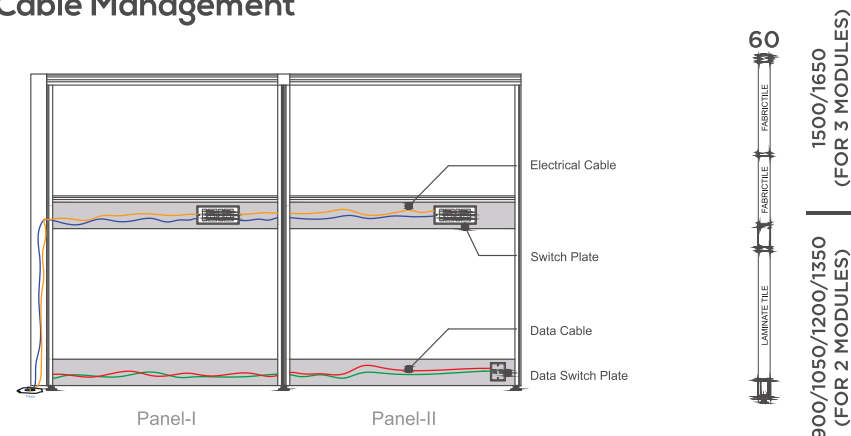
Data & Electrical cable Management-Below work surface
