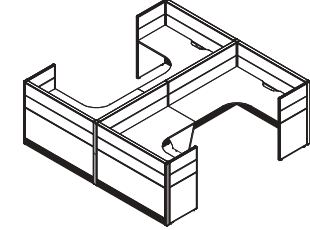
Curvilinear 4-pax cluster with 30mm transform panel C-Shaped
